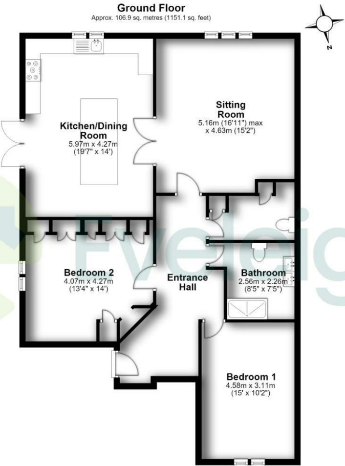
Total area: approx. 106.9 sq. metres (1151.1 sq. feet) Flat 5 Lons Court
